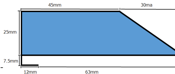
camSmart - View frame cross section
